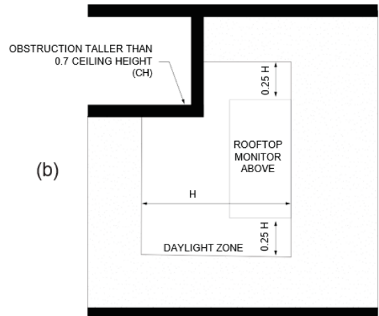
FIGURE C405.2.4.2(3) DAYLIGHT ZONE UNDER A SLOPED ROOFTOP MONITOR
