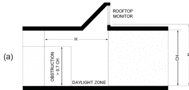
FIGURE C405.2.4.2(2) DAYLIGHT ZONE UNDER A ROOFTOP MONITOR
